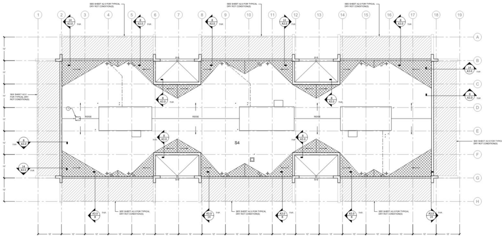
Roof Design Plans
